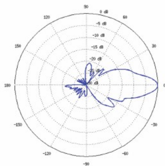
Horizontal Elevation
