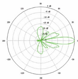
Horizontal Azimuth
