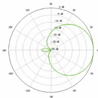
Horizontal Azimuth
