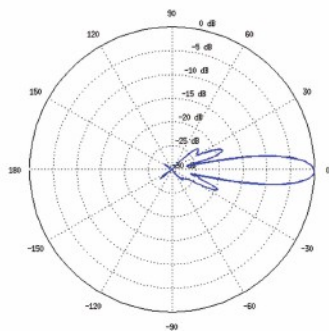
Vertical Elevation
